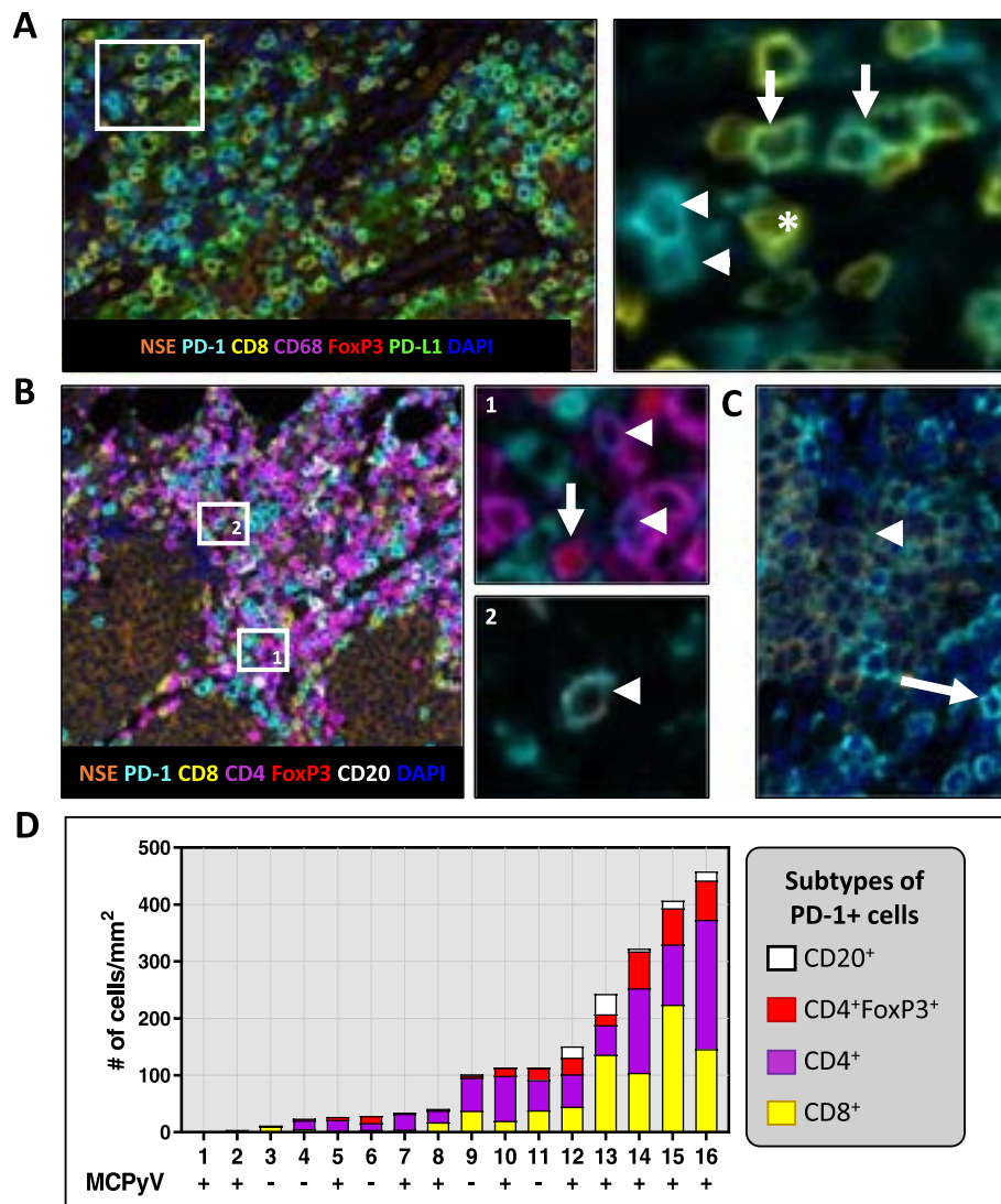
Fig. 4 Multiplex immunofluorescence studies demonstrate that PD-1 is expressed on multiple cell types in MCC, including CD8+ cells, CD4+ cells, T_{reg} (CD4 + FoxP3+), CD20+ B-cells, and even sometimes on tumor cells. a Representative photomicrograph of multiplex panel (CD8, yellow; CD68, magenta; FoxP3, red; NSE (tumor), orange; PD-1, cyan; PD-L1, green and DAPI) from a responder in the cohort of patients treated with anti-PD-1. Higher magnification photomicrograph shows that while there is a significant proportion of PD-1+/CD8+ cells (arrow), there are also PD-1+ cells that are CD8- (arrowhead), and CD8+ cells that are PD-1- (asterisk). Left and right panels: 200x and 400x original magnification, respectively. b A second multiplex panel (PD-1, cyan; CD8, yellow; CD4, magenta; FoxP3, red; CD20, white; NSE (tumor), orange, and DAPI) was applied to archival MCC specimens to further characterize cell types expressing PD-1. Left panel: Representative photomicrograph showing host-tumor interface, 200x original magnification. Upper-right panel (1): Cell types expressing PD-1 include CD4 + FoxP3+ cells (arrow) and PD-1 + FoxP3- (arrowhead) cells, 400x original magnification. Lower-right panel (2): CD20+ B-cells (arrowhead) were also noted to express PD-1. (only CD20 and PD-1 channels are shown in the inset, 400x original magnification). c In one case, low-level, constitutive PD-1 expression on nearly every tumor cell was observed (arrowhead). High levels of PD-1 expression were also seen on TIL (arrow). d PD-1+ cell densities across n = 16 tumor specimens show that PD-1 expression on multiple cell types is observed across different levels of inflammation. The virus status of each specimen is displayed below each specimen number
