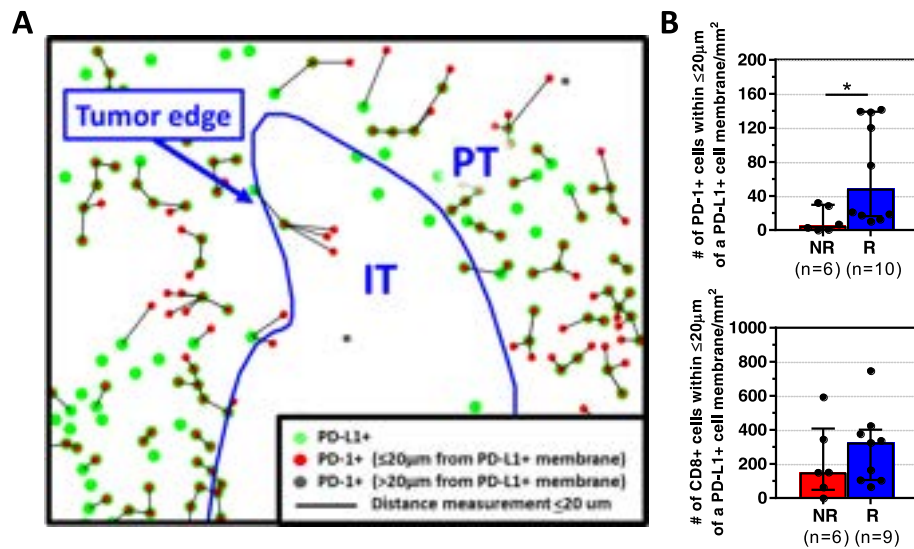
Fig. 3 The density of PD-1+ cells adjacent to a PD-L1+ cell correlates with clinical response to anti-PD-1. a Representative composite image depicting proximity analysis between PD-1+ and PD-L1+ cells performed using the HALO software Spatial Analysis module, Supplemental Methods. The distance between each PD-1+ cell and the nearest PD-L1+ cell (green circles) was calculated, and only those at a distance \leq 20 \mu\text{m} (black lines) are quantified (red circles). b Responders (R) had significantly higher median densities ( \pm\text{IQR} ) of PD-1+, but not CD8+, cells interacting with PD-L1+ cells compared to non-responders (NR). * p < 0.05 . The density of PD-L1+ cells within 20 \mu\text{m} of a PD-1+ or CD8+ cell was also calculated, and a similar association with response was observed, Additional file 1: Figure S6
